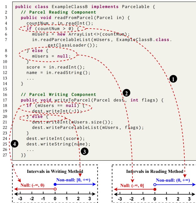
Figure 12: Interval mapping. ❶ and ❷ semantically convert the condition of the if-else control flow in the reading method to intervals. ❸ and ❹ semantically convert the condition of the if-else control flow in the writing method to intervals. Our analysis also supports if-else-if-else control flows.
