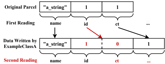
Figure 3: Data mismatches in ExampleClassA
